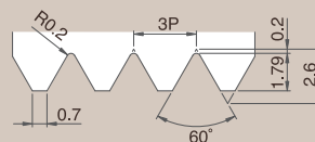
Pitch 3.0 齒型詳圖
